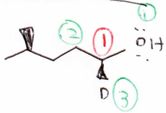
(S)-4-deutero-4-methylpentan-1-ol
