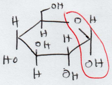
\alpha -D-glucopyranose
