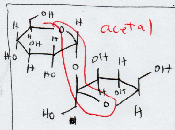
Sucrose
