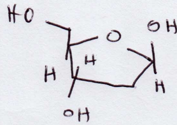
2-deoxyribose
