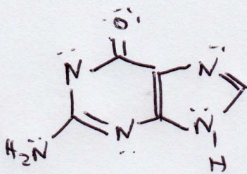
guanine
