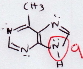
adenine
