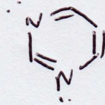
pyrimidine
